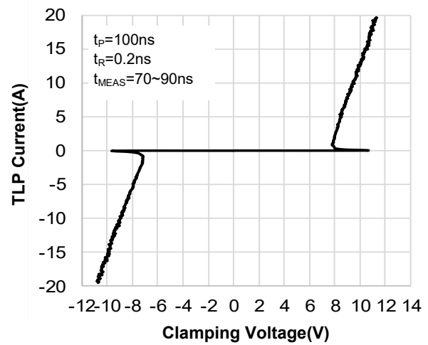
TLP Curve
