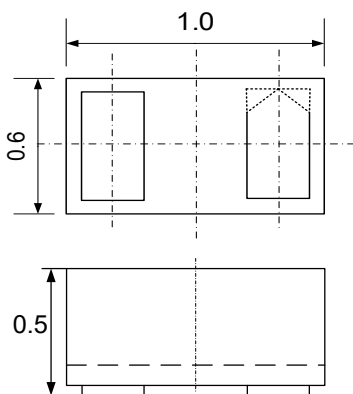
Package Dimensions
